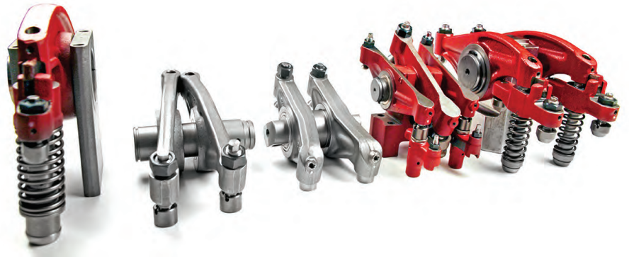
ROCKER ARM ASSEMBLY TYPE : HIMSEN / MAN / WARTSILA
